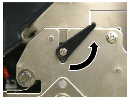
Pinch Roller Hebel
