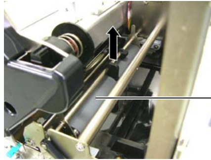
Pinch Roller Block
